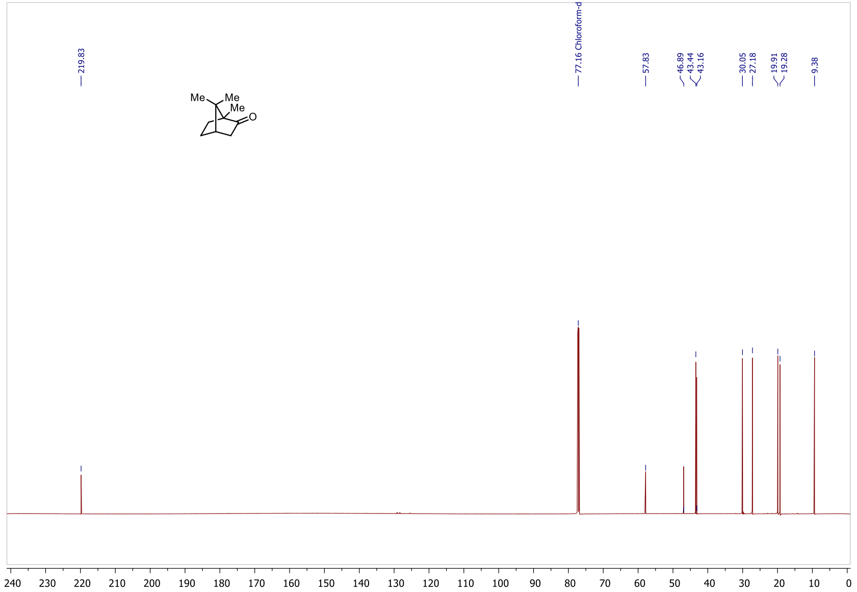
Figure 1. ^{13}\text{C-NMR} of 1 (176 MHz, \text{CDCl}_3 )
